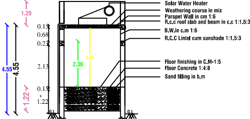
SECTION - "AB "
