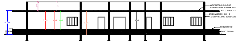
SECTION ON XX
