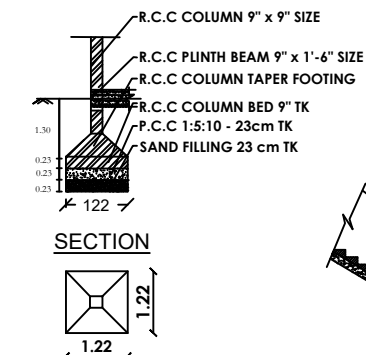
COLUMN DETAILS PLAN
