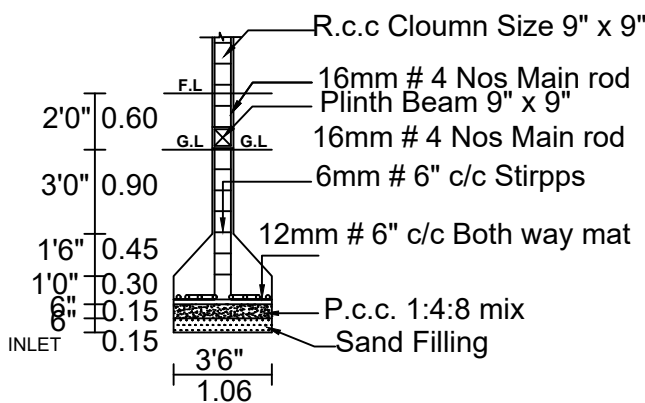
COLUMN DETIAL
