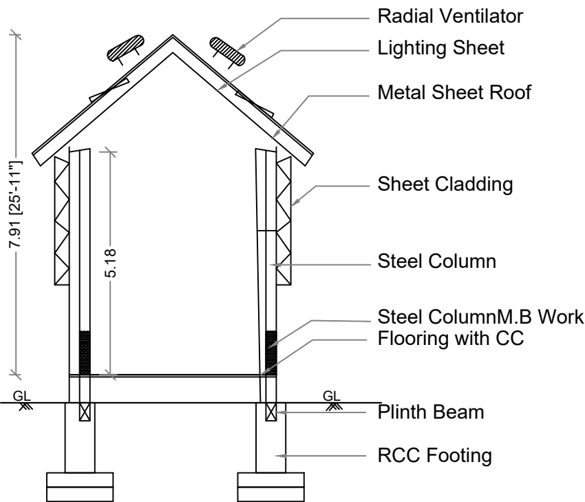
SECTION ON SHED A-B
