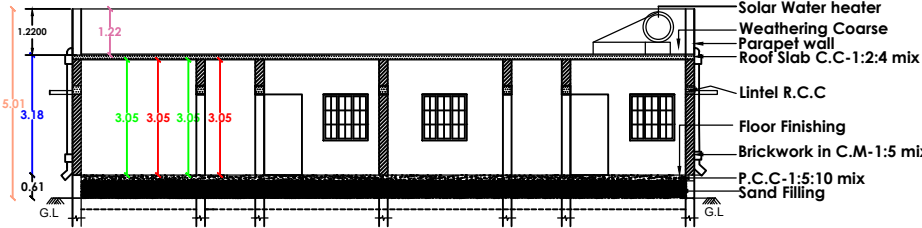
SECTION"AB"
