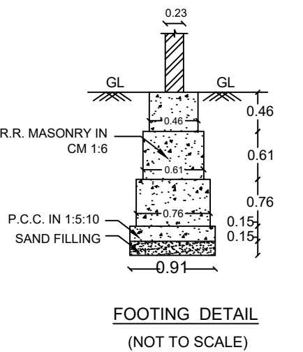
FOUNDATION DETAIL (NOT TO SCALE)
