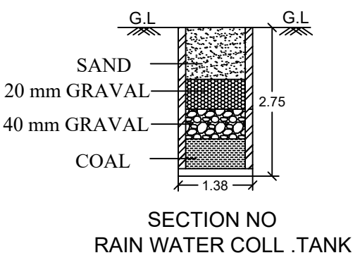
SECTION NO RAIN WATER COLL .TANK
