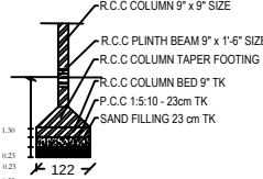
SECTION
