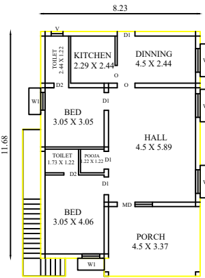
EXIST GROUND FLOOR PLAN
