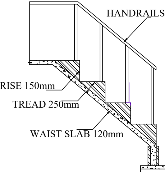
STAIRCASE DETAILS
