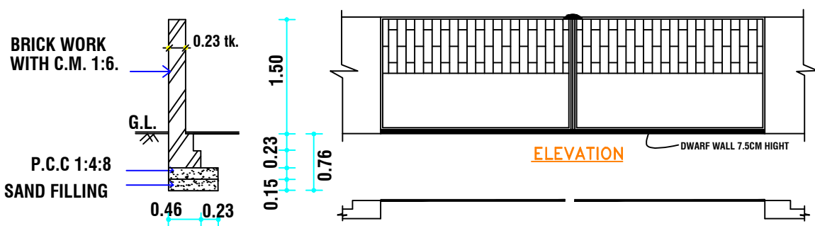
SECTION OF COMPOUND WALL
