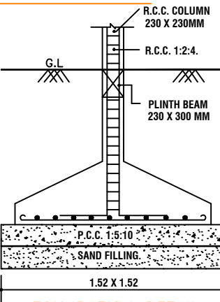
FOUNDATION DETAIL
