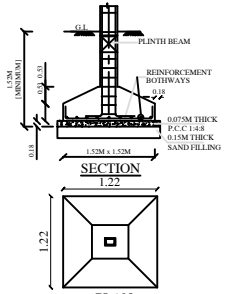
FOUNDATION DETAILS
