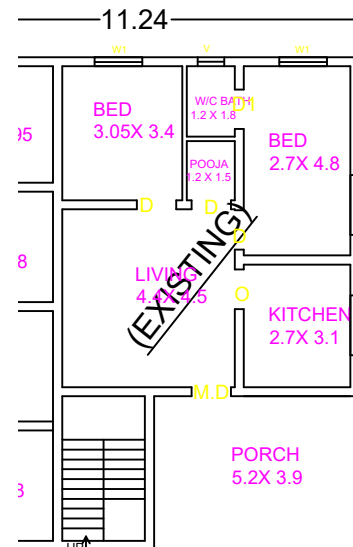
EXISTING GROUND FLOOR
