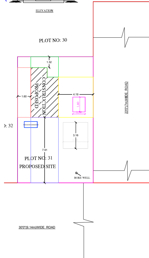
SITE PLAN
