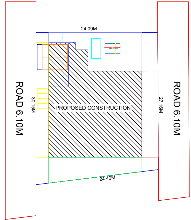
SITE PLAN
