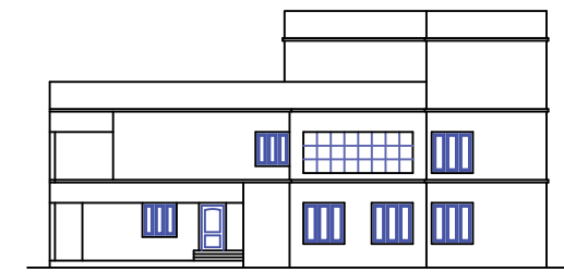
FRONT ELEVATION
