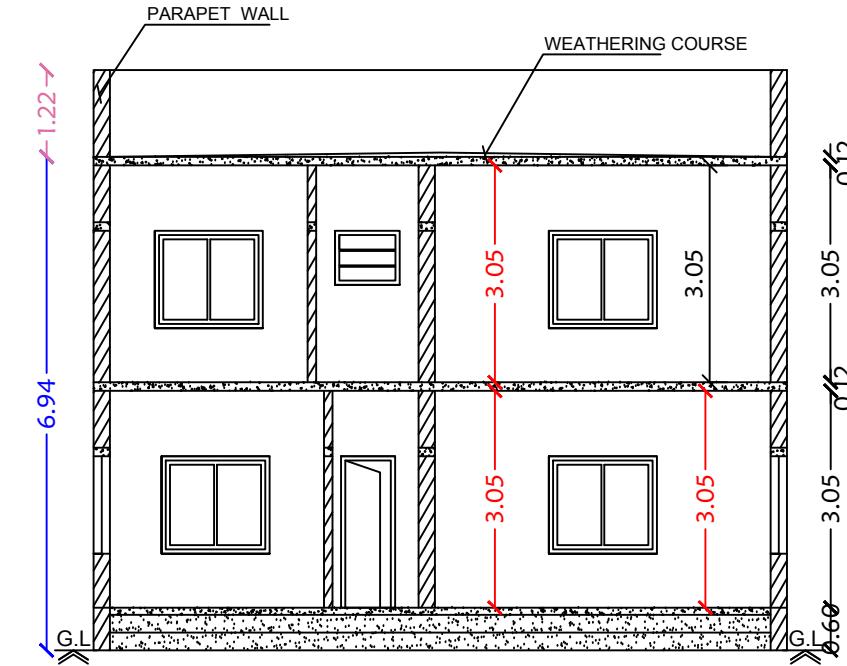
Section on-"AA"
