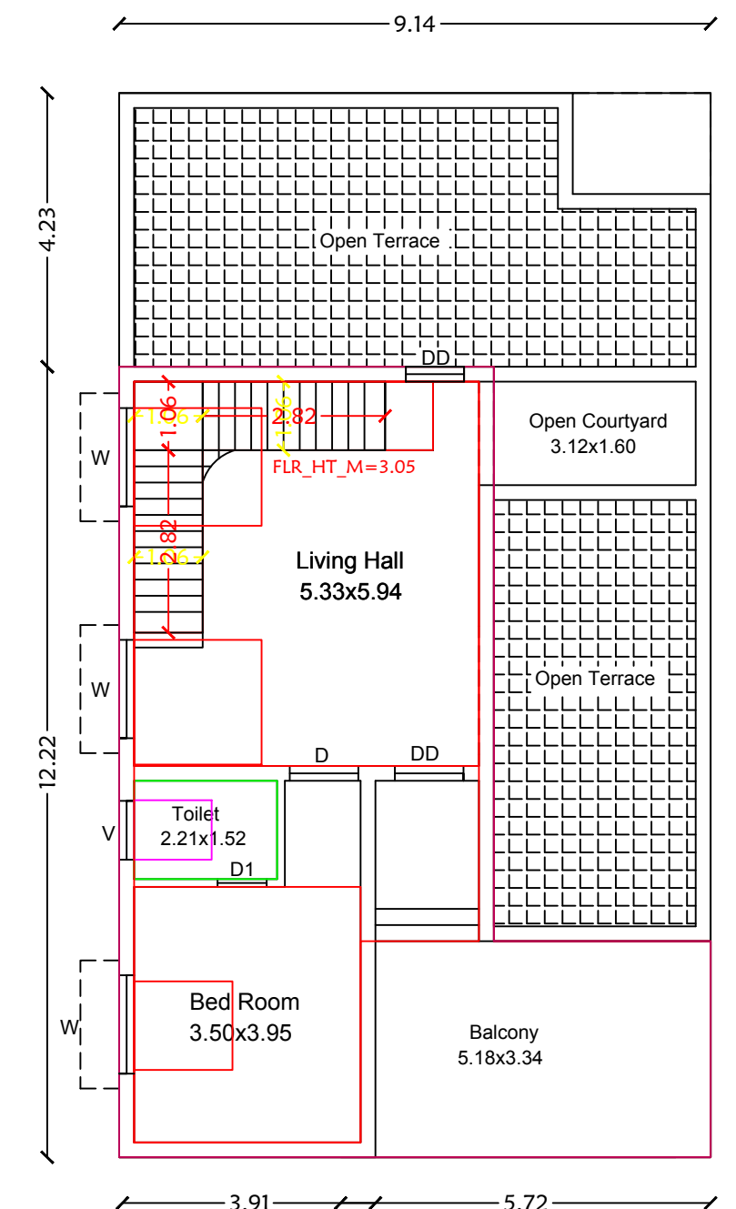
Ground Floor
