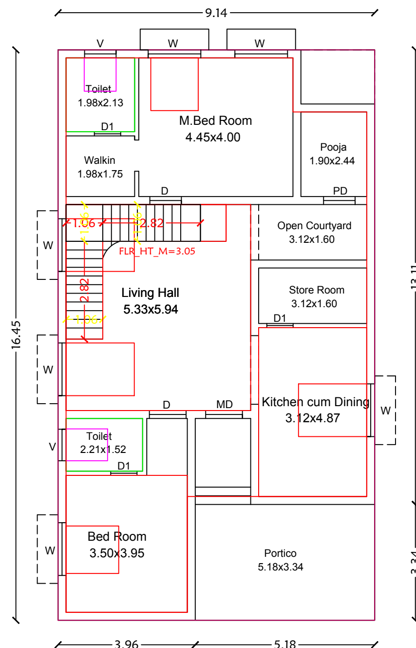
Ground Floor
