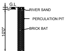
PERCOLATION PIT
