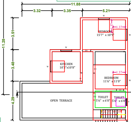
PRO.SECOND FLOOR PLAN
