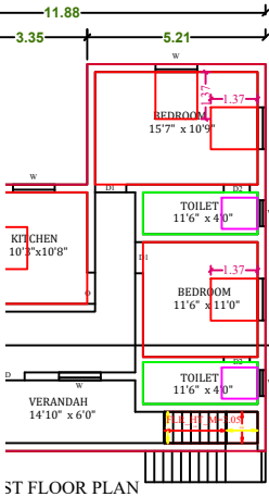
ST FLOOR PLAN
