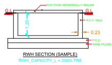
RWH SECTION (SAMPLE) RWH CAPACITY, L = 2000LTRS
