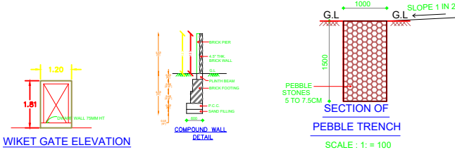
WIKET GATE ELEVATION
