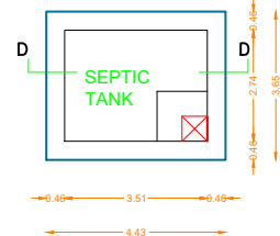
PLAN OF SEPTIC TANK
