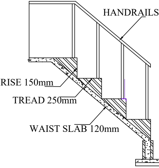
STAIRCASE DETAILS
