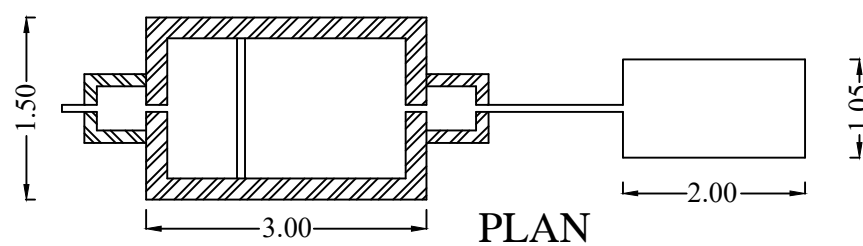
SEPTIC TANK DISPERSION TRENCH
