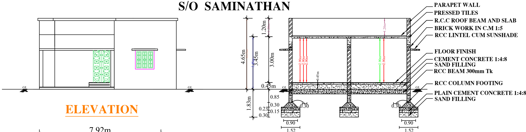
SECTION [A-A]
