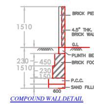
COMPOUND WALLDETAIL
