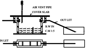
DETAILS OF SEPTICTANK & D-TRENCE
