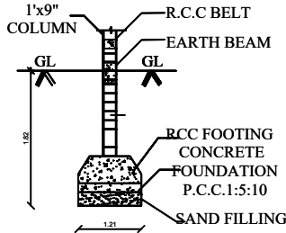
FOUNDATION DETAILS
