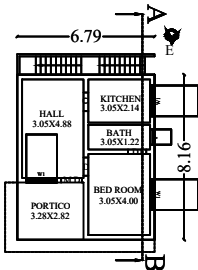
PROPOSED GROUND FLOOR PLAN
