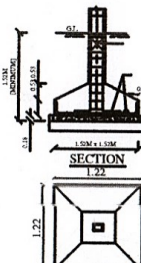
FOUNDATION DETAILS
