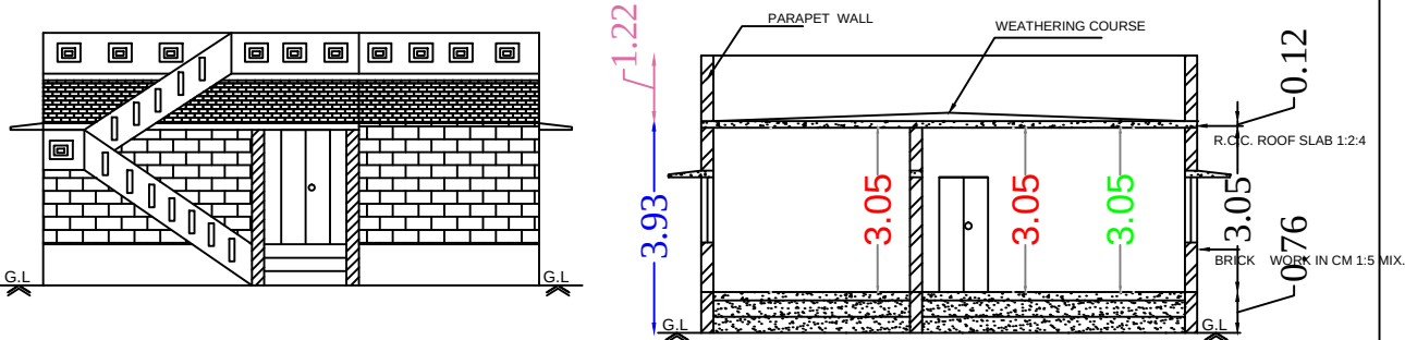
Front Elevation
