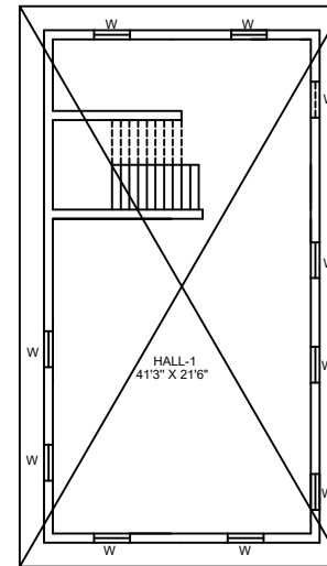
PROPOSED SECOND FLOOR PLAN
