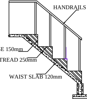
STAIRCASE DETAILS
