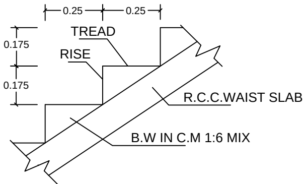
SECTION OF STAIRCASE
