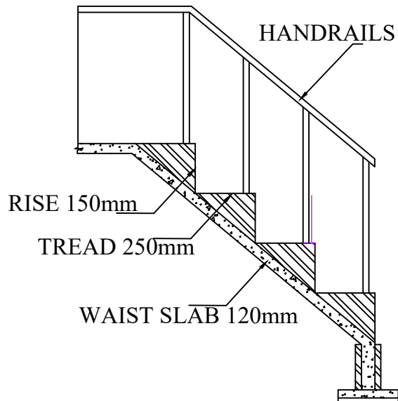
STAIRCASE DETAILS
