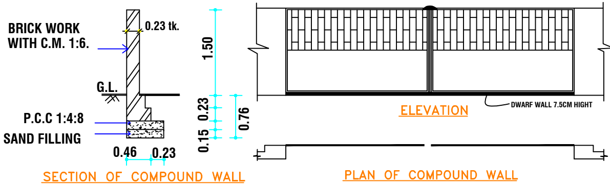
SECTION OF COMPOUND WALL
