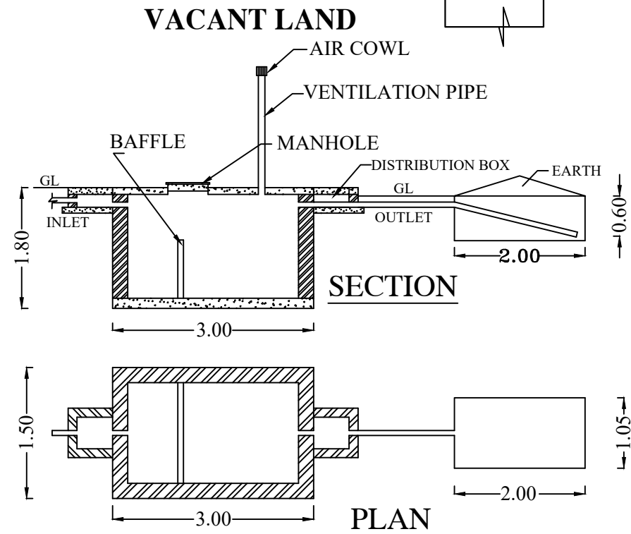
SEPTIC TANK DISPERSION TRENCH
