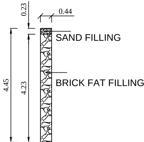
DETAILS OF PERCOLATION PIT
