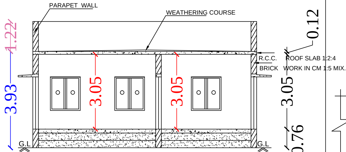
Section on-AA
