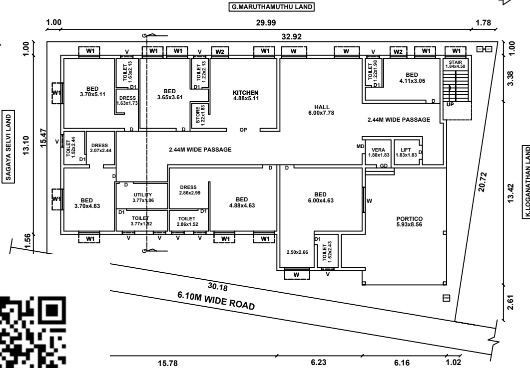
SITE CUM GROUND FLOOR PLAN
