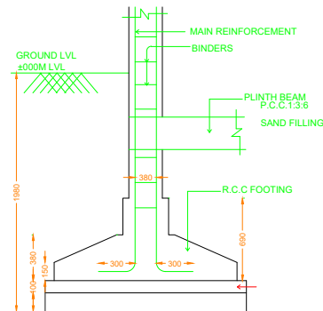
TYPICAL SECTION OF R.C.C COLUMN FOUNDATION SCALE : 1\"/>
