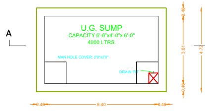
SUMP DETAIL SCALE 1\"/>
