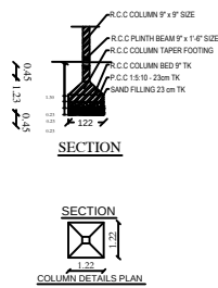
COLUMN DETAILS PLAN
