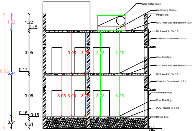
SECTION - "AB"
