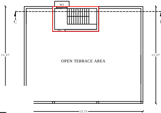
TERRACE FLOOR
