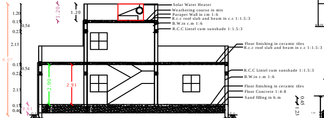
SECTION - "AB-CD"
