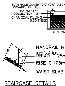
STAIRCASE DETAILS
