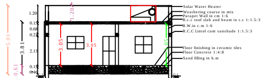
SECTION - "AB "
