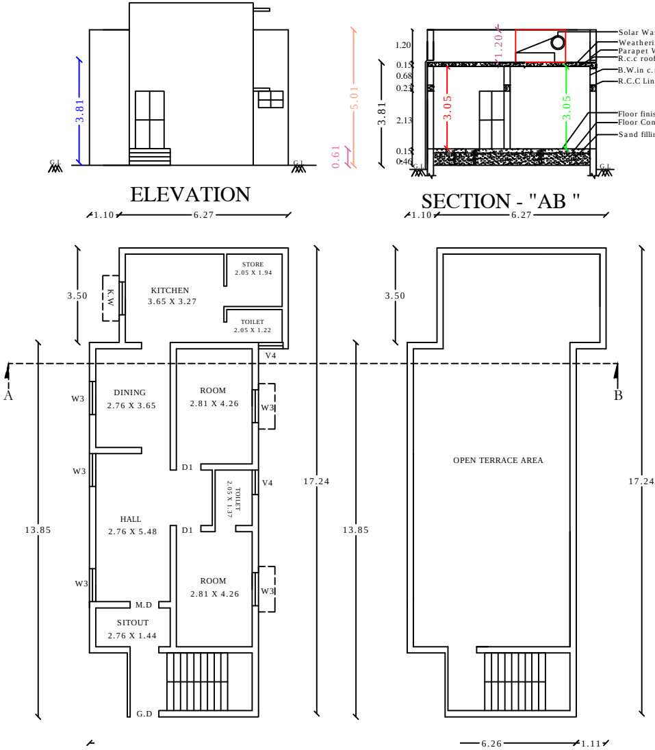
TERRACE FLOOR
