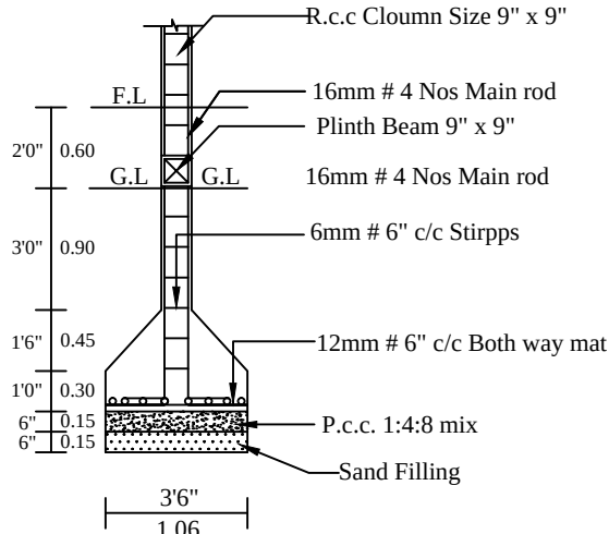
COLUMN DETIALS
