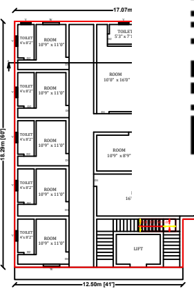
EXG.GROUND FLOOR PLAN
