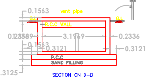
SECTION ON D-D
