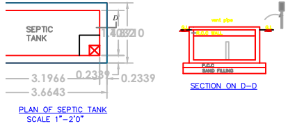
PLAN OF SEPTIC TANK SCALE 1\"/>
