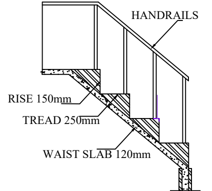
STAIRCASE DETAILS
