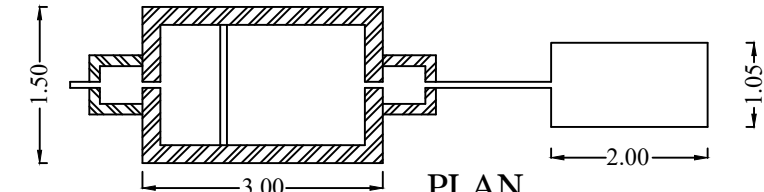
SEPTIC TANK DISPERSION TRENCH
