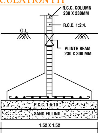
FOUNDATION DETAIL
