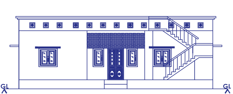
FRONT ELEVATION
