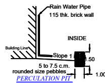
RAIN WATER PIPE
