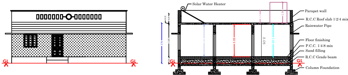
FRONT ELEVATION
