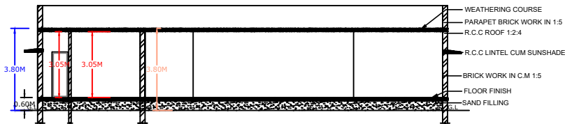
SECTION ON XX
