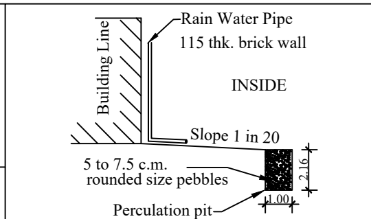
RAIN WATER HARVESTING PERCOLATION PIT
