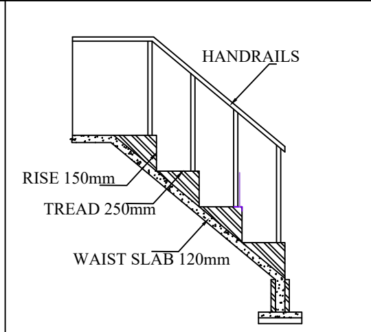
STAIRCASE DETAILS
