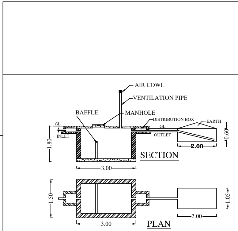
SEPTIC TANK DISPERSION TRENCH
