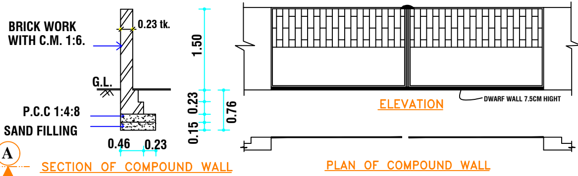
COMPOUND WALL
