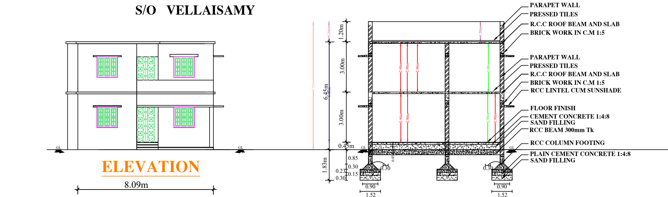
SECTION [A-A]
