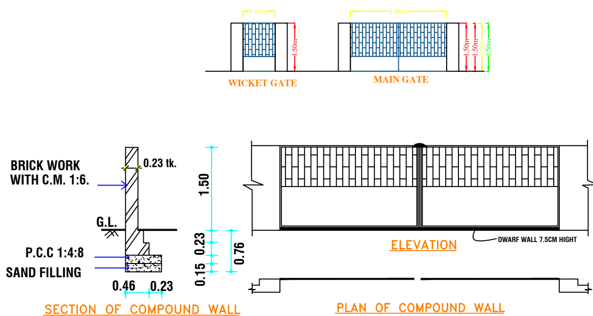
SECTION OF COMPOUND WALL
