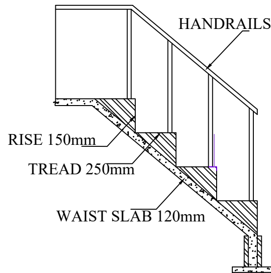
STAIRCASE DETAILS
