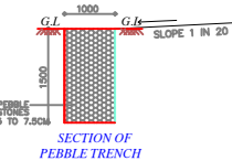
SECTION OF PEBBLE TRENCH
