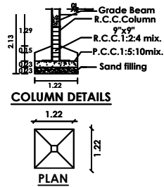
COLUMN DETAILS
