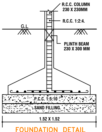
FOUNDATION DETAIL
