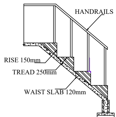
STAIRCASE DETAILS
