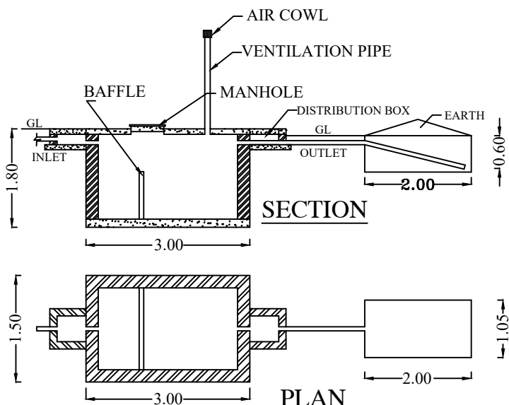
SEPTIC TANK DISPERSION TRENCH
