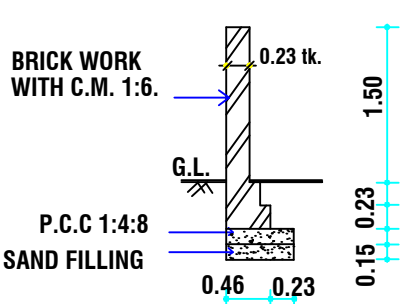
SECTION OF COMPOUND WALL
