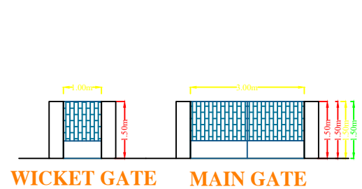
WICKET GATE MAIN GATE
