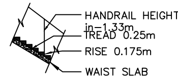
STAIRCASE DETAILS
