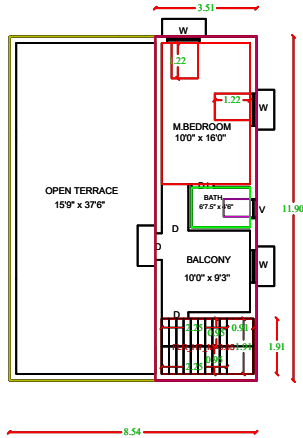
PRO. FIRST FLOOR PLAN.
