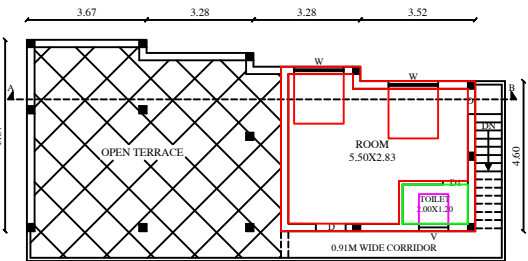
PRO. SECOND FLOOR PLAN
