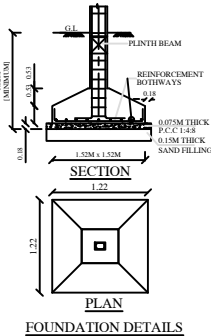
FOUNDATION DETAILS
