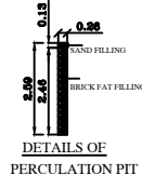
DETAILS OF PERCUSSION PIT
